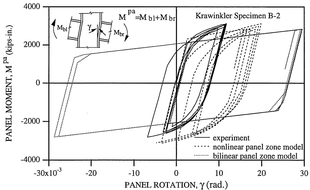
Fig. 7.4d: Comparison of Experimental and Analytical Panel Moment-Rotation Relations of Krawinkler Specimen B-2 (Krawinkler 1971).
