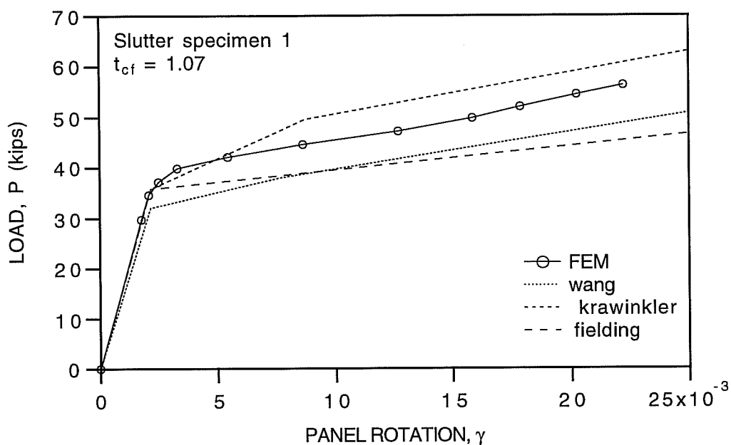
Fig. 5.14: Comparison of the Existing Models and FEM Result for Slutter Specimen 1 with t_{cf} = 1.07
