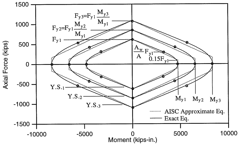
Fig. 2.7: Initial and Subsequent Yield Surfaces
