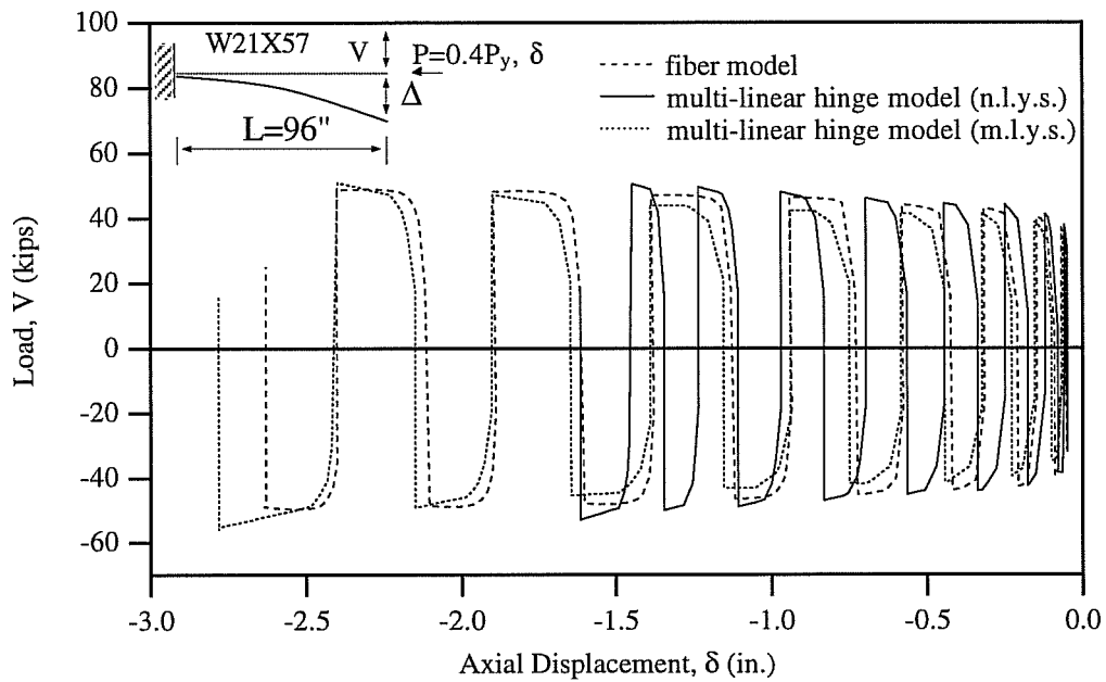
Fig. 4.45d: Comparison of Transverse Load-Axial Deformation Relationships Obtained by the Multi-Linear Hinge and Fiber Models for P = 0.4P_y .
