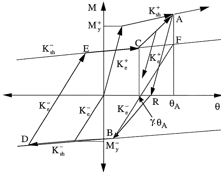
Fig. 6.2: Moment-Rotation Hysteresis Model of Composite Beam (Lee 1987)
