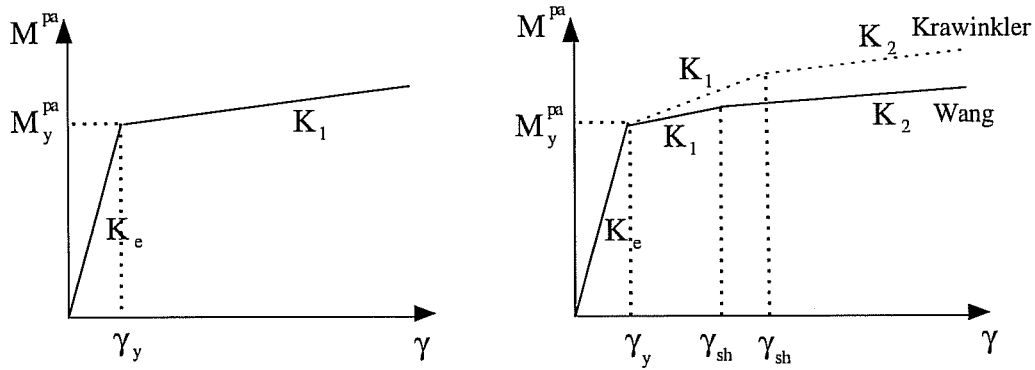
a) Fielding's Bilinear Model b) Krawinkler and Wang's Trilinear Models
