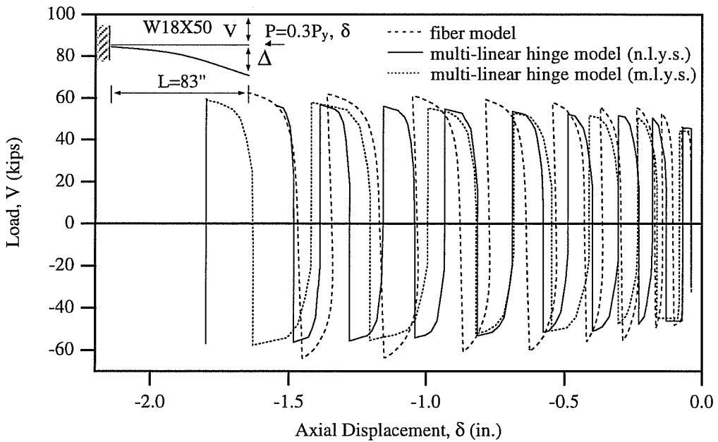
Fig. 4.48d: Comparison of Transverse Load-Axial Deformation Relationships Obtained by the Multi-Linear Hinge and Fiber Models for P = 0.3P_y .
