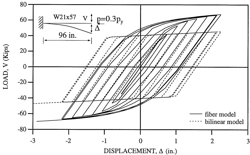
Fig. 2.2: Comparison of Kanaan's Hinge Model with Fiber Model
