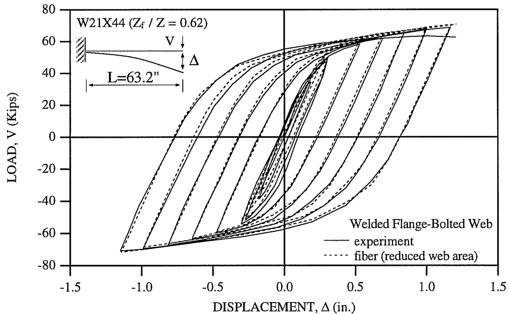
Fig. 4.15: Comparison of Experimental Results and Predictions Made by the Fiber Model for Tsai Specimen 18.
