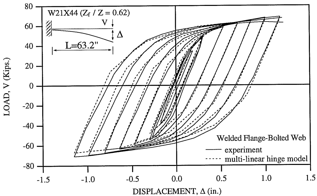
Fig. 4.26: Comparison of Experimental Results and Predictions Made by the Multi-Linear Hinge Model for Tsai Specimen 18.
