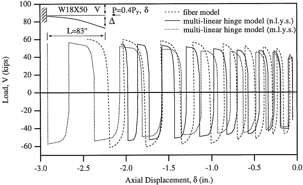
Fig. 4.49d: Comparison of Transverse Load-Axial Deformation Relationships Obtained by the Multi-Linear Hinge and Fiber Models for P = 0.4P_y .
