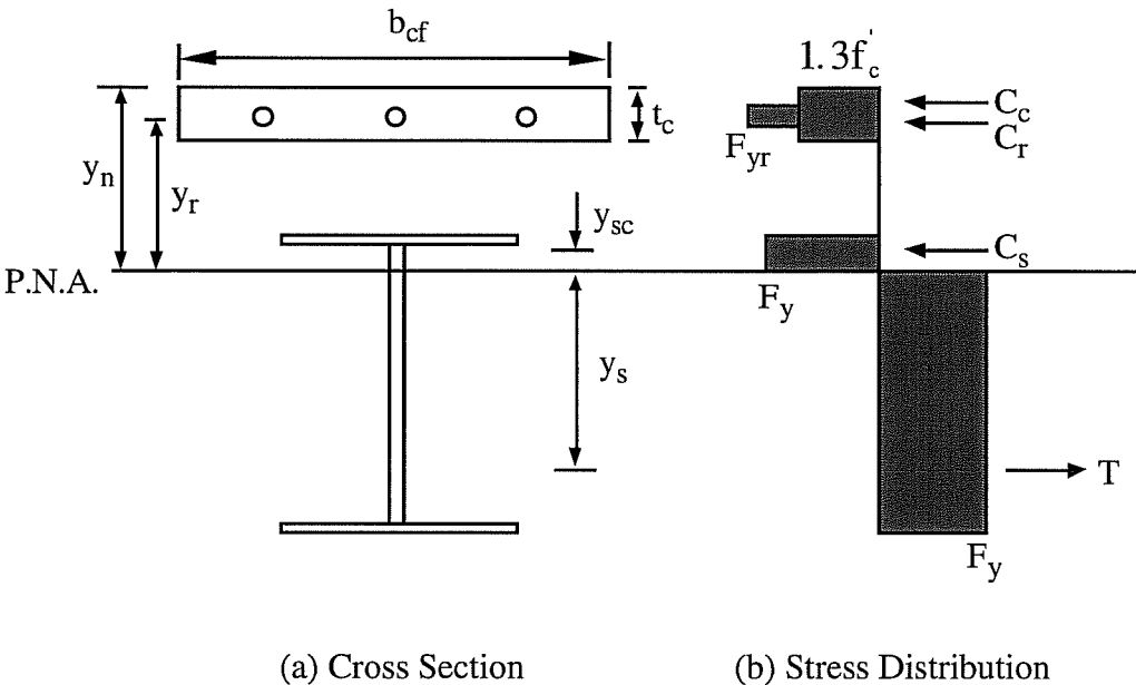
Fig. 6.3: Plastic Stress Distribution of Composite Beam.
