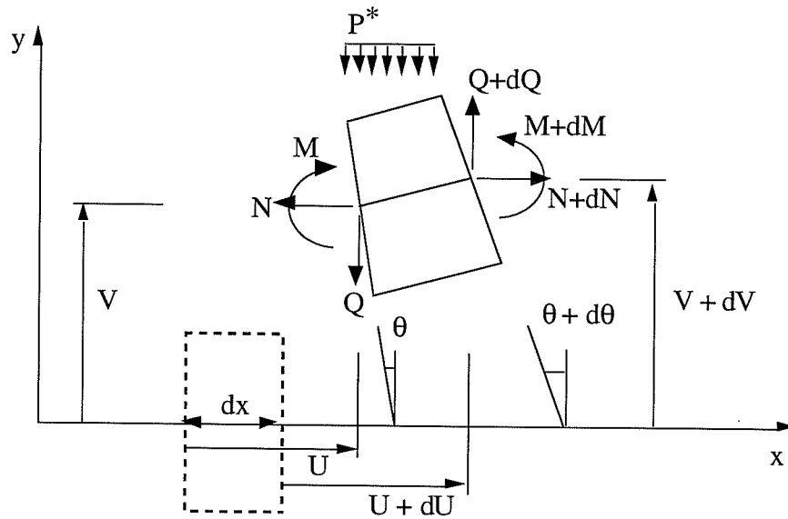
Fig. 3.3: Second Order Equilibrium of a Beam Slice
