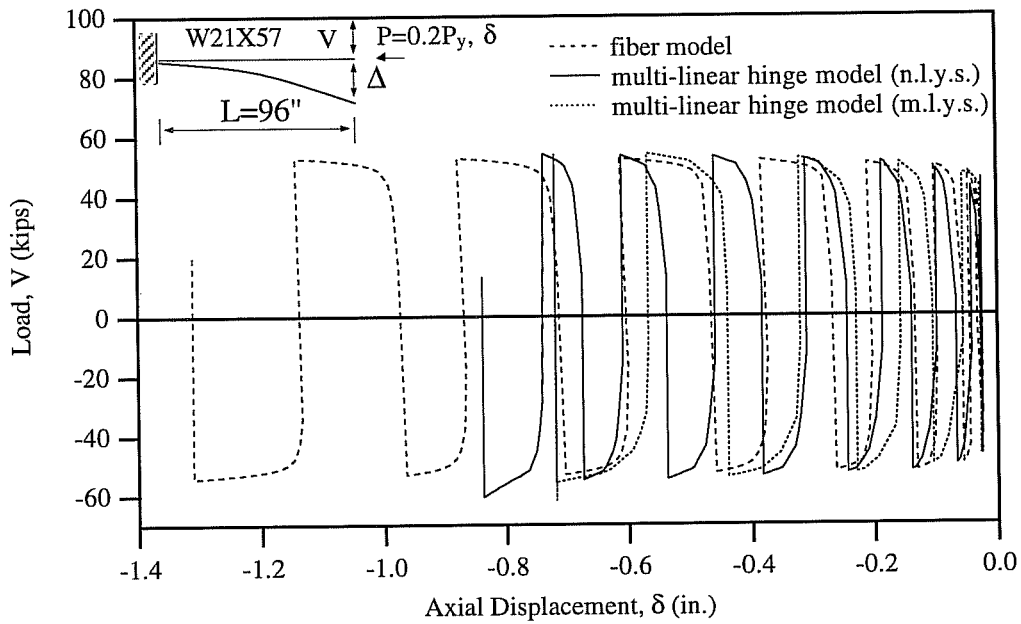
Fig. 4.43d: Comparison of Transverse Load-Axial Deformation Relationships Obtained by the Multi-Linear Hinge and Fiber Models for P = 0.2P_y .
