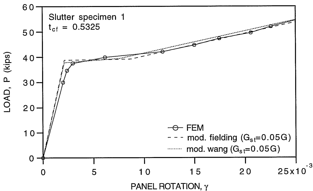
Fig. 5.22: Comparison of the Modified Models and FEM Result for Slutter Specimen 1 with t_{cf} = 0.5325 ”
