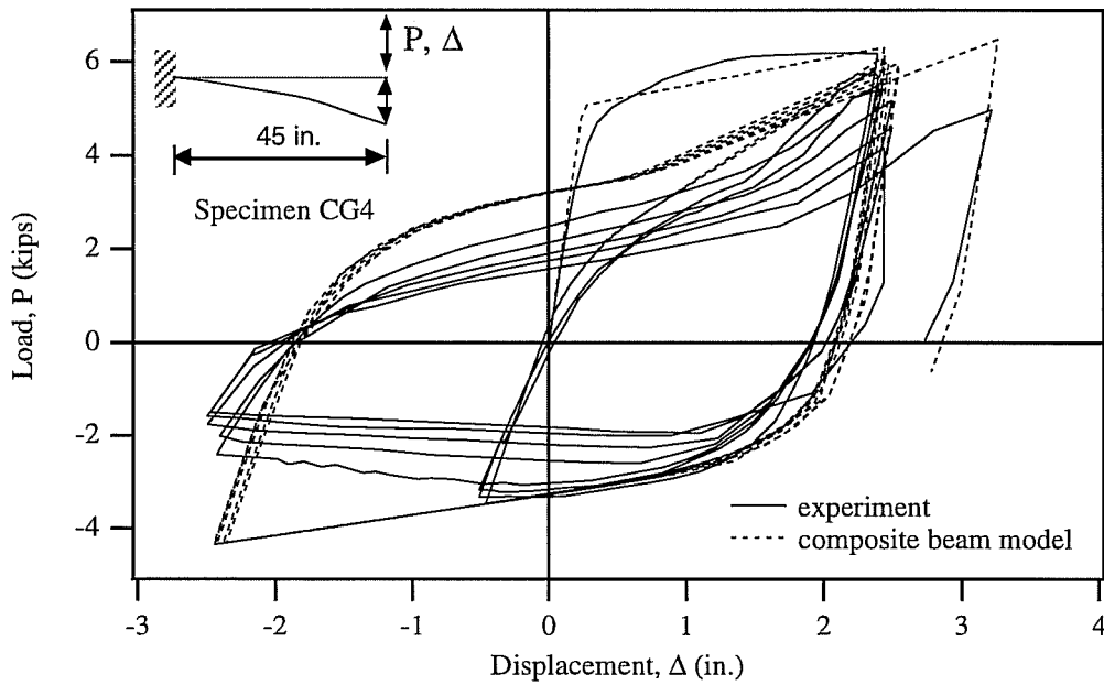
Fig. 6.10: Comparison of Experimental and Analytical Results of Specimen CG4
