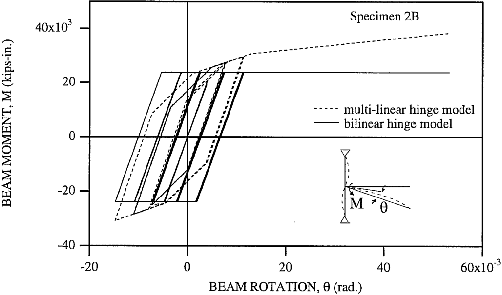
Fig. 7.10c: Comparison of Analytical Beam Moment-Rotation Relations of Engelhardt Specimen 2B (Engelhardt 1994).
