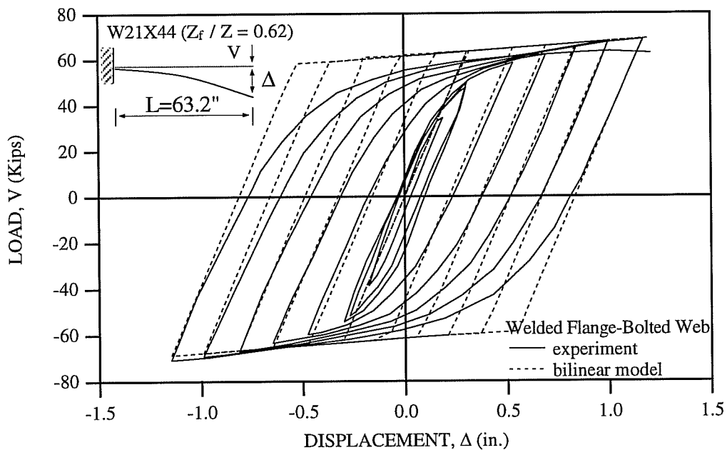
Fig. 4.19: Comparison of Experimental Results and Predictions Made by Bilinear Model for Popov Specimen 4.
