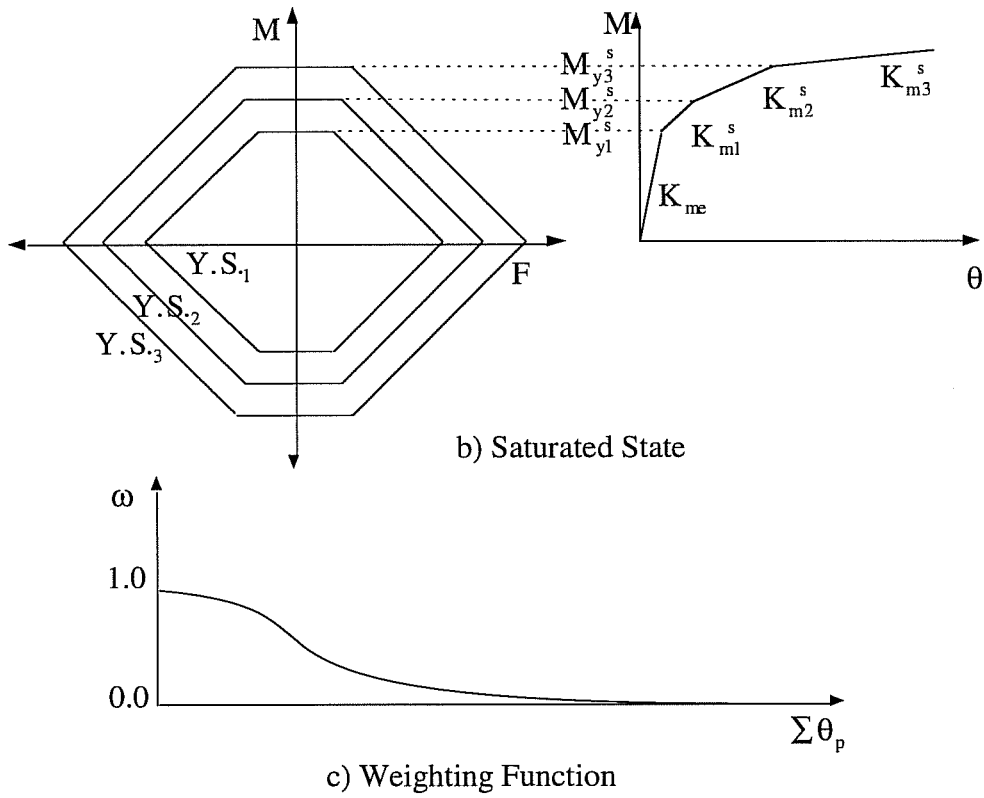
Fig. 2.13: Typical Moment-Rotation Curves for Two Limiting States
