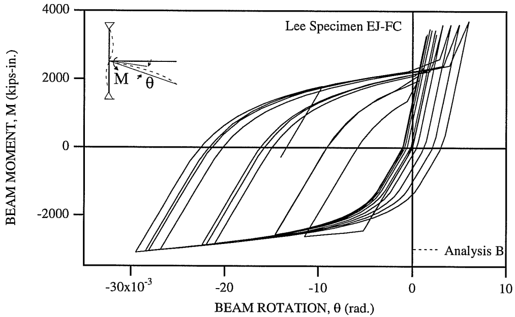
Fig. 7.19c: Beam Moment-Rotation Relation Obtained by the Analysis Using the Parameters for the Panel Zone of the Exterior Composite Beam-to-Column Joints (Lee 1987).
