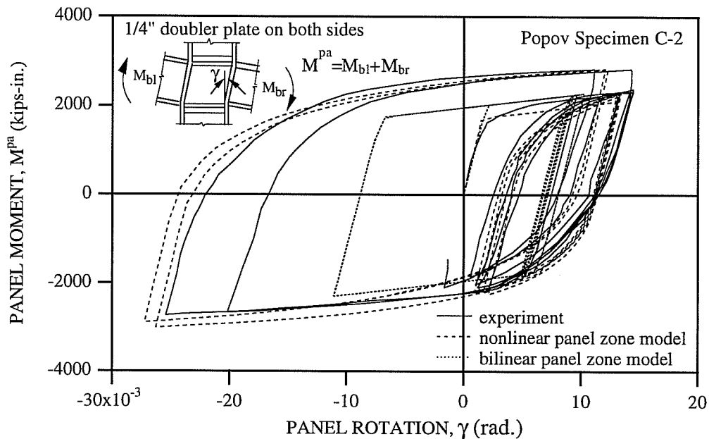
Fig. 7.11f: Comparison of Analytical Panel Moment-Rotation Relations of Popov Specimen C-2 (Popov 1975).
