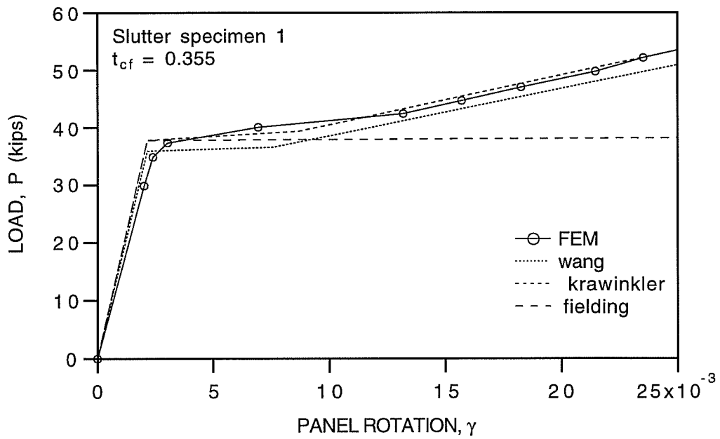
Fig. 5.11: Comparison of the Existing Models and FEM Result for Slutter Specimen 1 with t_{cf} = 0.355
