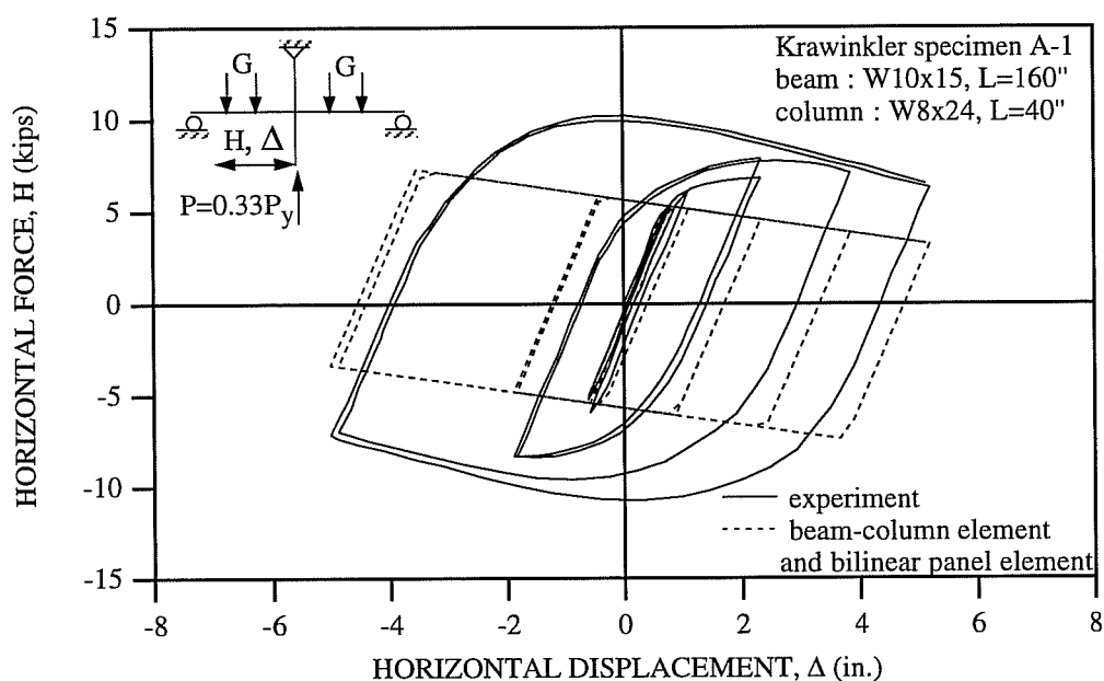
Fig. 5.28: Comparison of Test and the Analysis Using the Bilinear Panel Model for Overall Response
