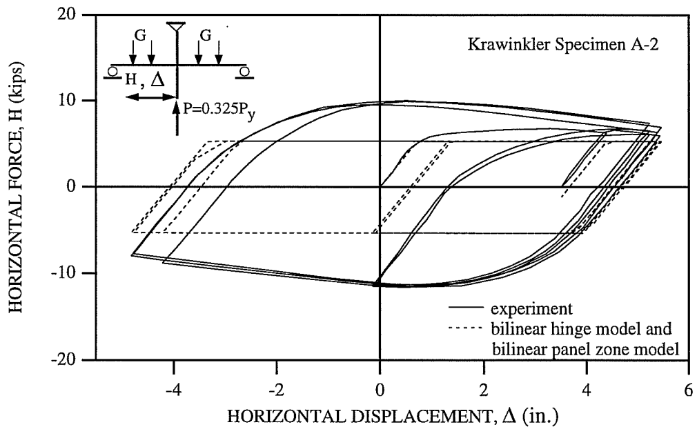
Fig. 7.2b; Comparison of Experimental and Analytical Results Obtained by Bilinear Hinge Model and Bilinear Panel Zone Model for Krawinkler Specimen A-2 (Krawinkler 1971).
