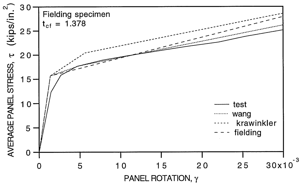
Fig. 5.9: Comparison of the Existing Models and Test Data for Fielding Specimen
