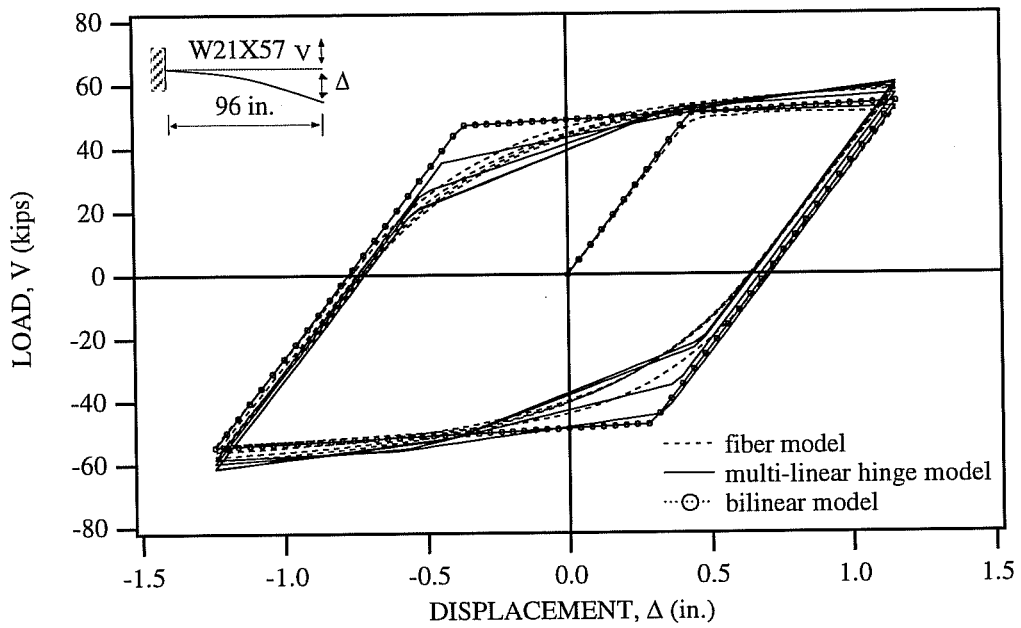
Fig. 4.31: Comparison of the Multi-Linear Hinge Model and Other Models for Displacement History No. 2
