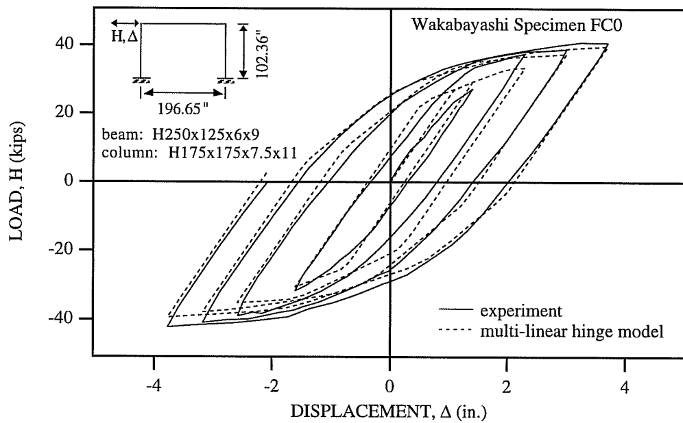
Fig. 7.13a: Comparison of Experimental Results and Analytical Prediction Made by Multi-linear Hinge Model for Wakabayashi Specimen FC0 (Wakabayashi 1974).
