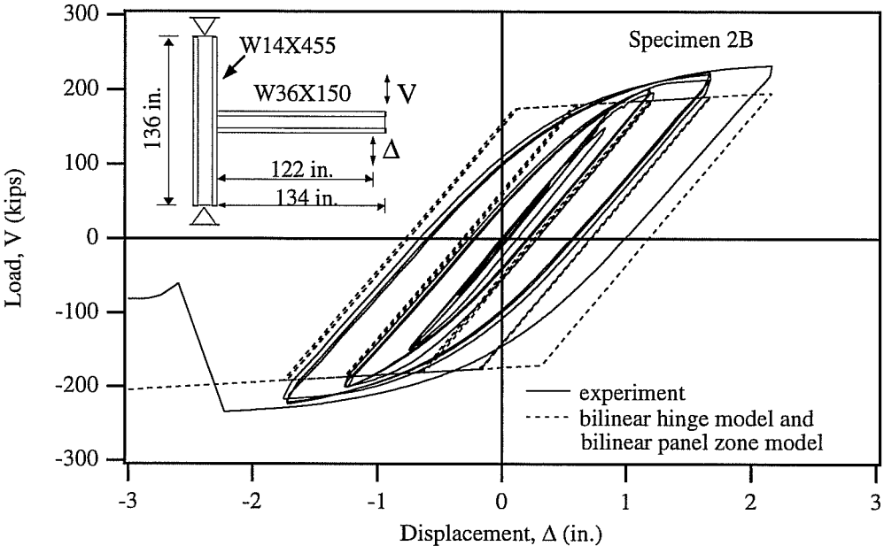
Fig. 7.10b: Comparison of Experimental and Analytical Results Obtained by Bilinear Hinge Model and Bilinear Panel Zone Model for Engelhardt Specimen 2B (Engelhardt 1994).
