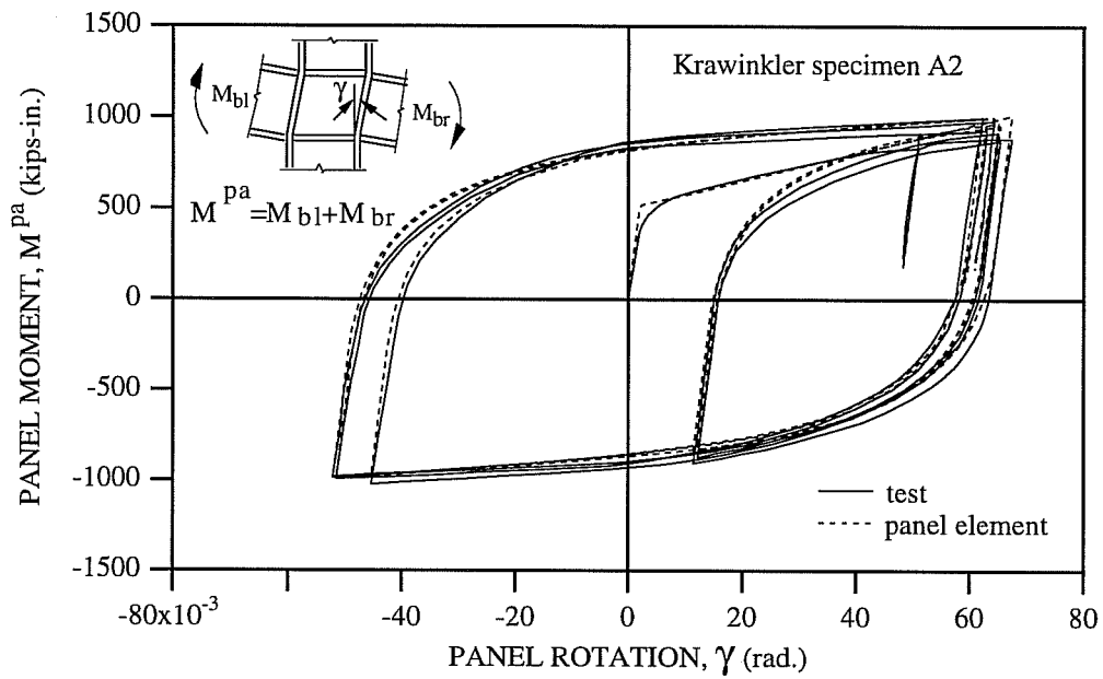
Fig. 5.33: Comparison of the Developed Hysteretic Rules and Test Data for Krawinkler Specimen A2
