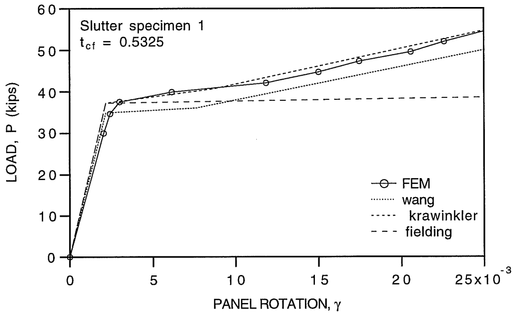
Fig. 5.12: Comparison of the Existing Models and FEM Result for Slutter Specimen 1 with t_{cf} = 0.5325 "
