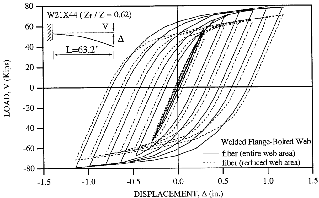
Fig. 4.18: Comparison of the Predictions Made by the Fiber Model for Tsai Specimen 18 With and Without the Reduced Web Area.
