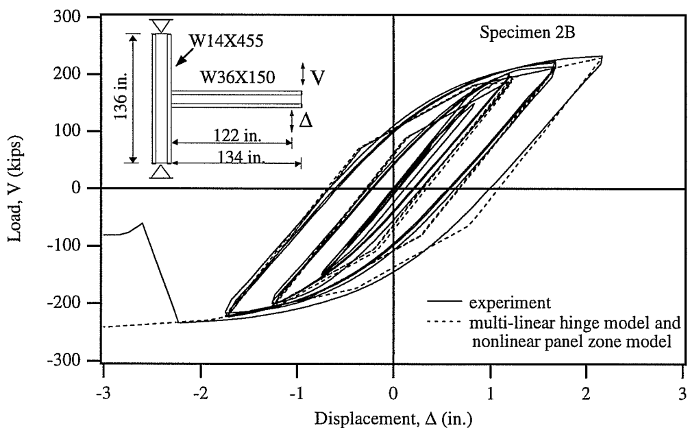
Fig. 7.10a: Comparison of Experimental and Analytical Results Obtained by Multi-linear Hinge Model and Nonlinear Panel Zone Model for Engelhardt Specimen 2B (Engelhardt 1994).
