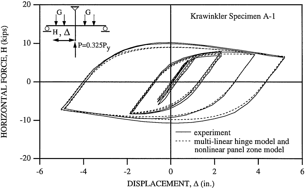
Fig. 7.1a: Comparison of Experimental and Analytical Results Obtained by Multi-linear Hinge Model and Nonlinear Panel Zone Model for Krawinkler Specimen A-1 (Krawinkler 1971).
