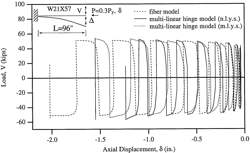
Fig. 4.44d: Comparison of Transverse Load-Axial Deformation Relationships Obtained by the Multi-Linear Hinge and Fiber Models for P = 0.3P_y .
