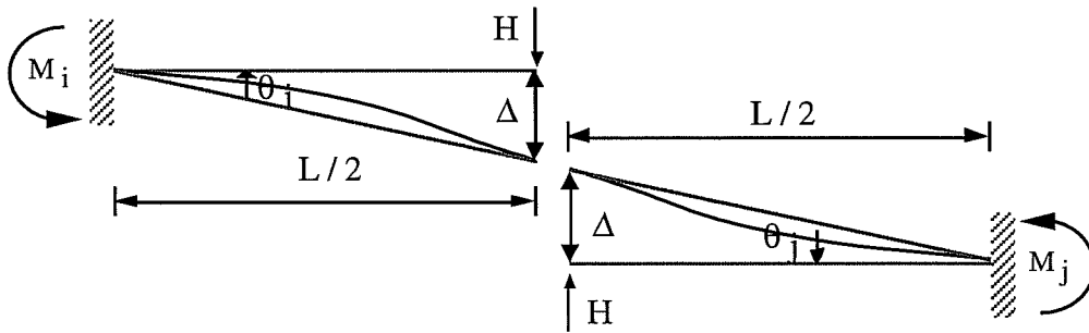
b) Equivalent Cantilevers
