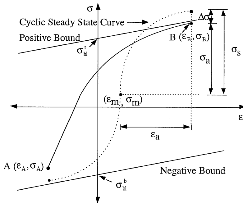
Fig. 3.8: Movement of Bound Line
