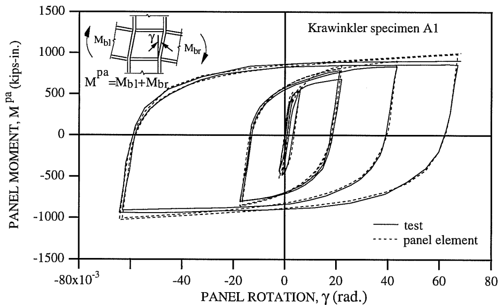
Fig. 5.32: Comparison of the Developed Hysteretic Rules and Test Data for Krawinkler Specimen A1
