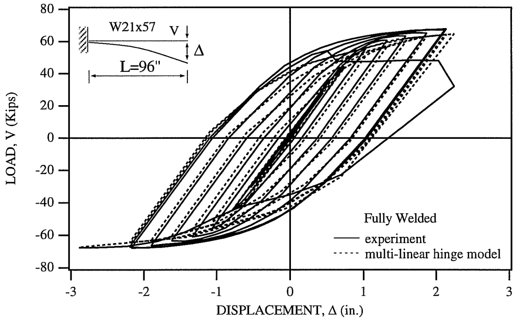
Fig. 4.9 Comparison of Experimental Results and Predictions Made by the Multi-Linear Hinge Model for Engelhardt Specimen 8.
