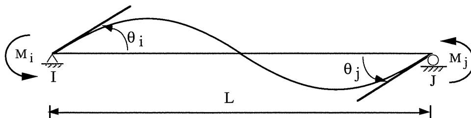
a) Beam with Equal End Moments
