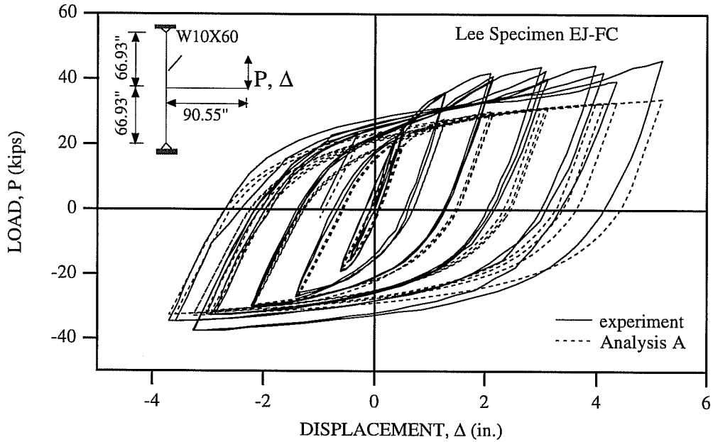
Fig. 7.16b: Comparison of Overall Response Obtained by the Test and the Analysis Using the Material Parameters of Bare Steel Beam-to-Column Joint for Lee Specimen EJ-FC (Lee 1987).
