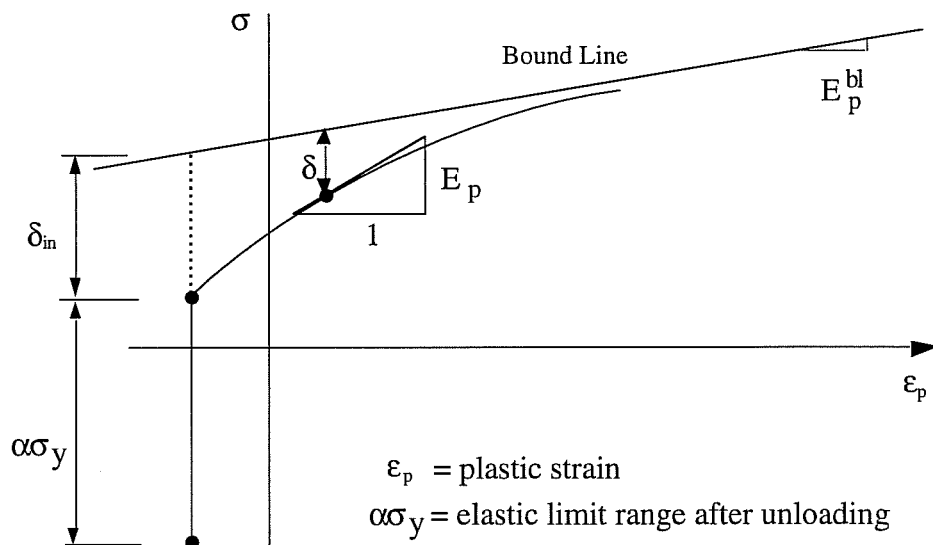
Fig. 3.9: Dafalias-Popov Model for Hysteresis Curve.
