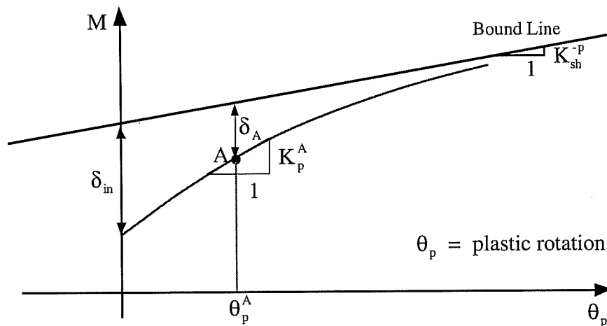
Fig. 6.5: Plastic Stiffness of Inelastic Moment-Rotation Curve
