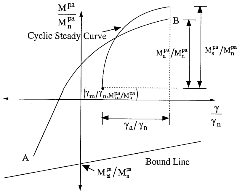
Fig. 5.30b): Movement of Bound Line
