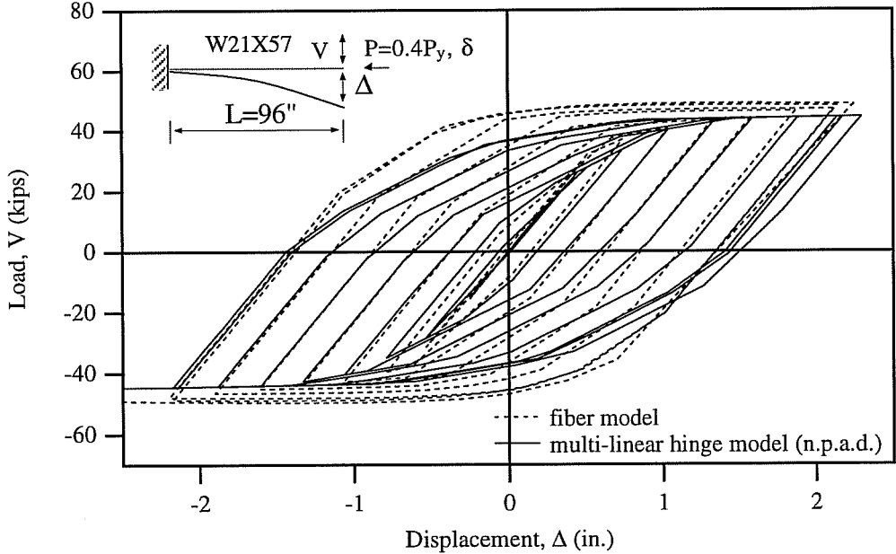
Fig. 4.45a: Comparison of Predicted Results by Fiber Model and Multi-Linear Hinge Model Neglecting Plastic Axial Deformations for P = 0.4P_y .
