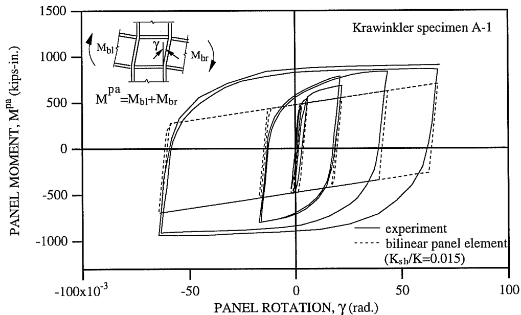
Fig. 5.27: Comparison of Test Results and the Existing Bilinear Panel Model for the Panel Zone
