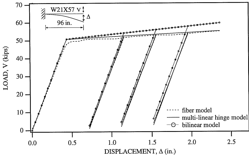
Fig. 4.30: Comparison of the Multi-Linear Hinge Model and Other Models for Displacement History No. 1
