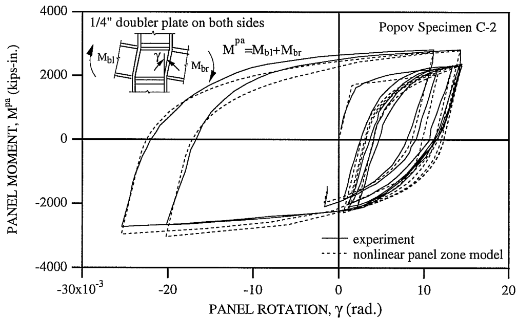
Fig. 7.11a: Comparison of Experimental Results and Analytical Panel Moment-Rotation Relations Obtained by Nonlinear Panel Zone Model for Popov Specimen C-2 (Popov 1975).
