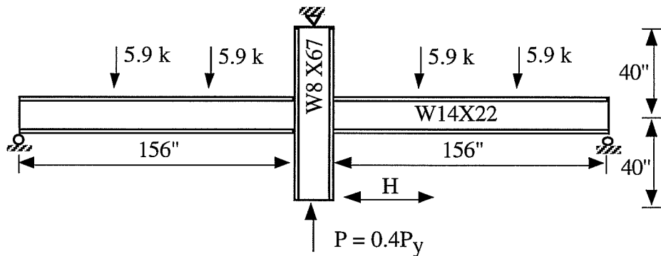
Fig. 5.6b): Krawinkler's Specimen B
