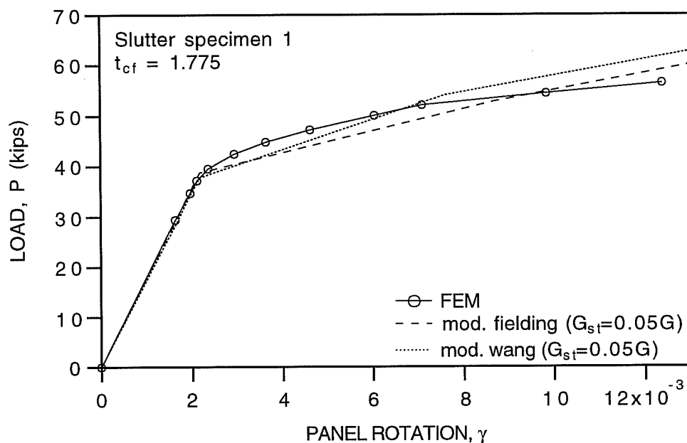
Fig. 5.26: Comparison of the Modified Models and FEM Result for Slutter Specimen 1 with t_{cf} = 1.775 ”
