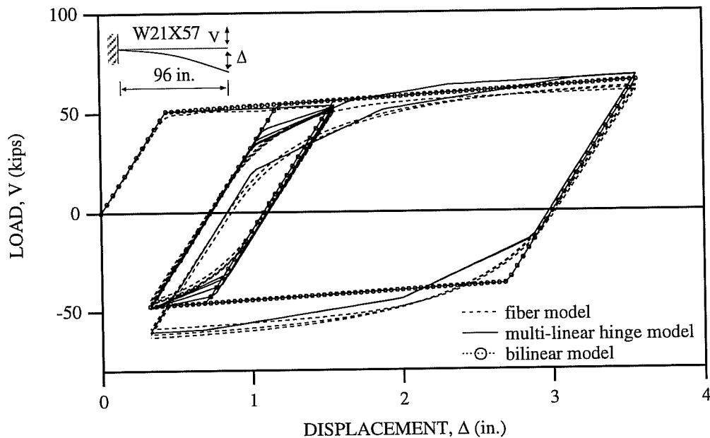
Fig. 4.35: Comparison of the Multi-Linear Hinge Model and Other Models for Displacement History No. 6
