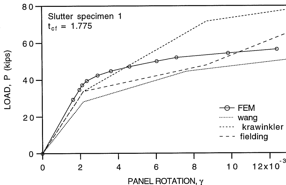
Fig. 5.16: Comparison of the Existing Models and FEM Result for Slutter Specimen 1 with t_{cf} = 1.775 "
