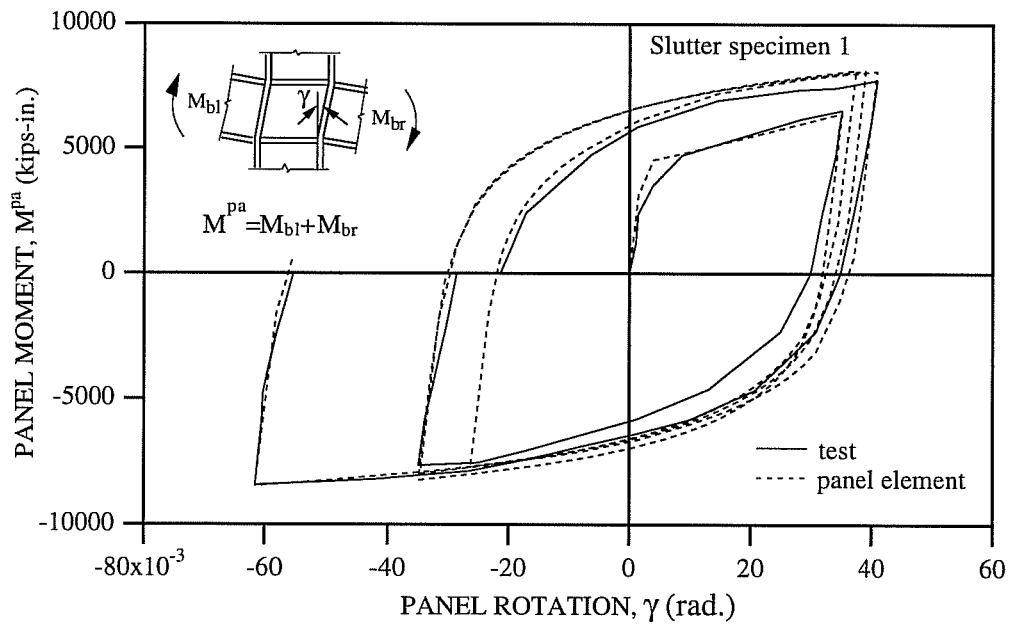
Fig. 5.36: Comparison of the Developed Hysteretic Rules and Test Data for Slutter Specimen 1
