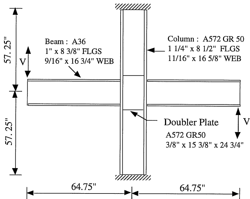
Fig. 5.31a): Slutter Specimens 2 and 4 (Slutter 1980)
