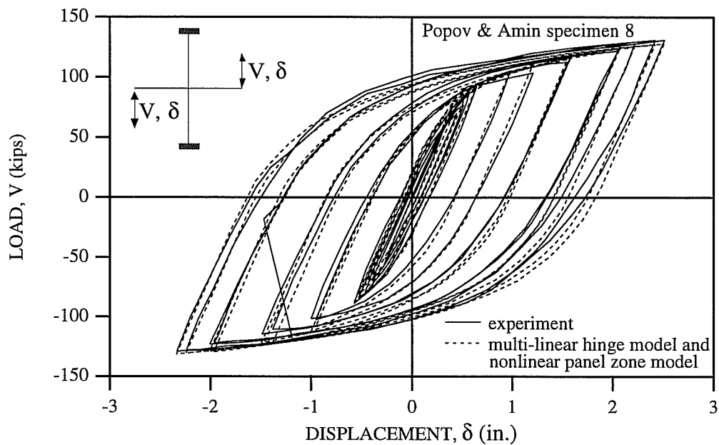
Fig. 7.9a: Comparison of Experimental and Analytical Results Obtained by Multi-linear Hinge Model and Nonlinear Panel Zone Model for Popov Specimen 8 (Popov 1985).
