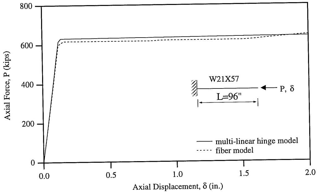
Fig. 4.36: Comparison of Multi-Linear Hinge Model and Fiber Model for Monotonic Axial Loading
