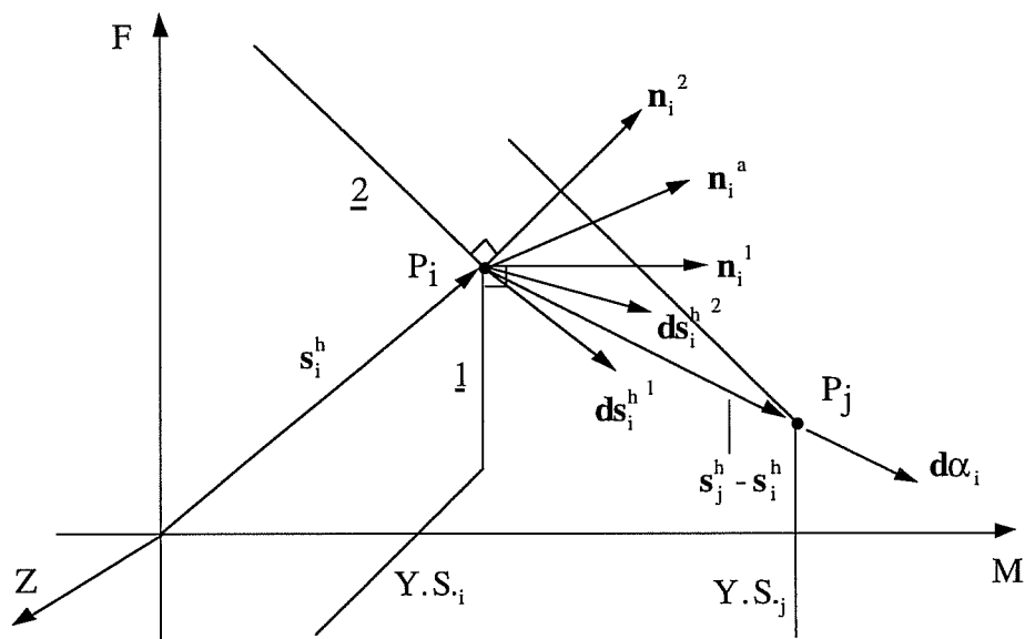
Fig. 2.21: Normal Vector at a Vertex of Yield Surface
