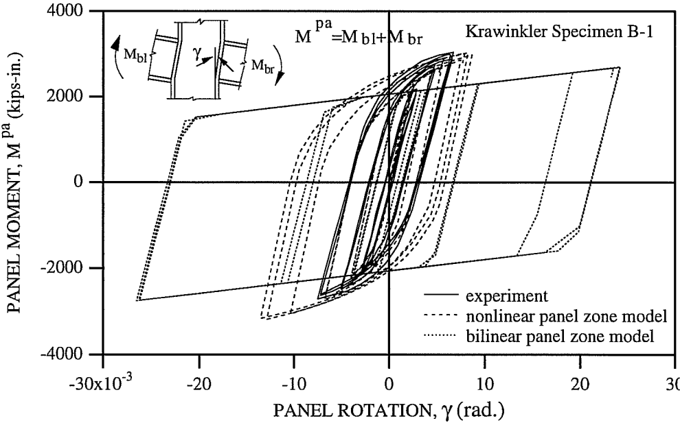
Fig. 7.3d: Comparison of Experimental and Analytical Panel Moment-Rotation Relations of Krawinkler Specimen B-1 (Krawinkler 1971).
