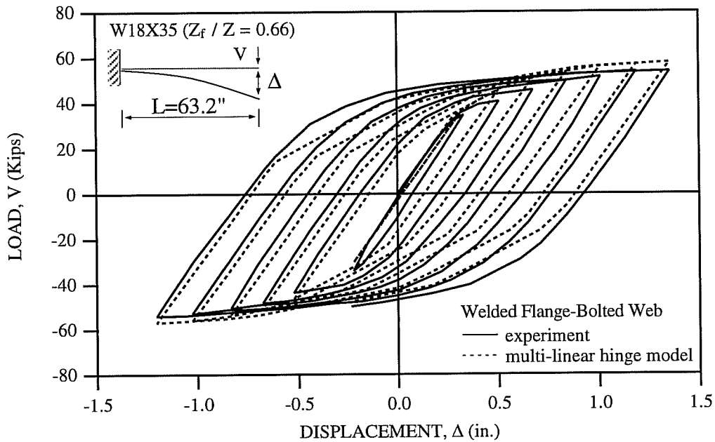
Fig. 4.25: Comparison of Experimental Results and Predictions Made by the Multi-Linear Hinge Model for Tsai Specimen 17.
