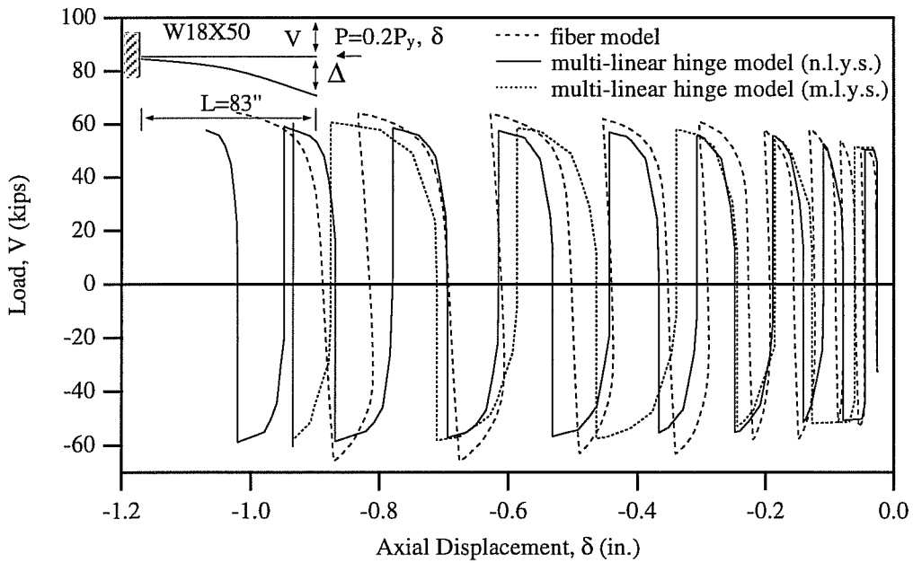
Fig. 4.47d: Comparison of Transverse Load-Axial Deformation Relationships Obtained by the Multi-Linear Hinge and Fiber Models for P = 0.2P_y .
