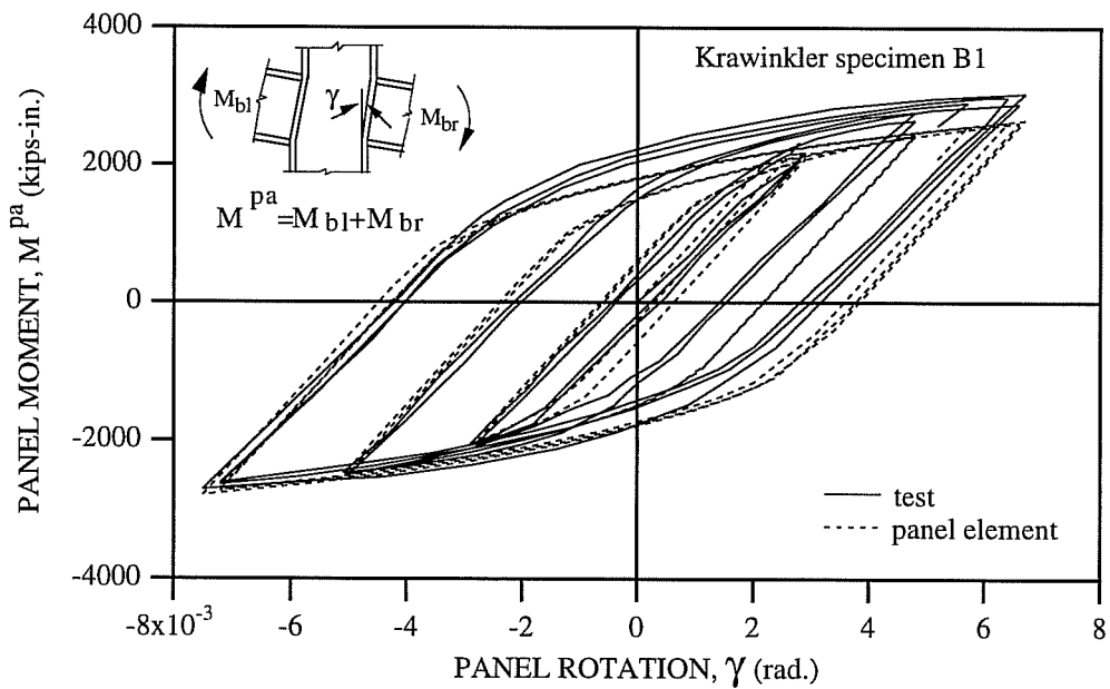
Fig. 5.34: Comparison of the Developed Hysteretic Rules and Test Data for Krawinkler Specimen B1
