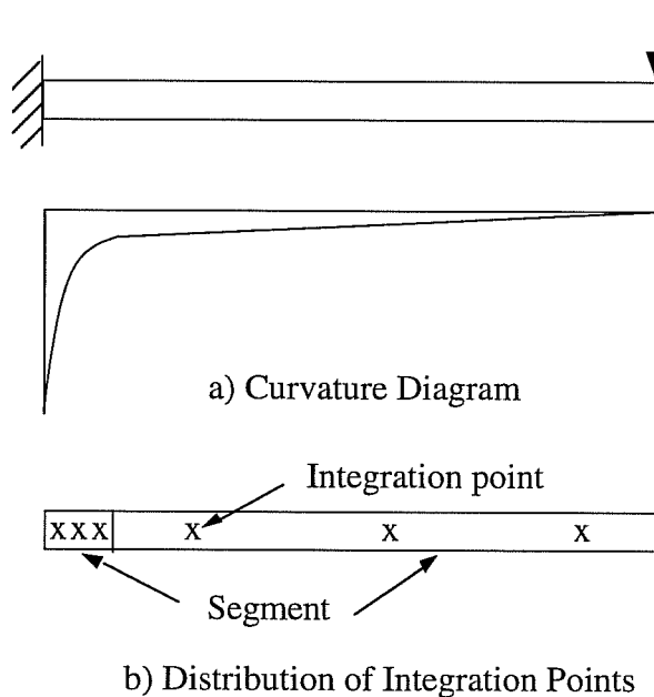
Fig. 3.5: Distribution of Integration Points Along Segments
