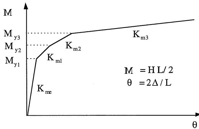
c) Moment-Rotation Relationship
