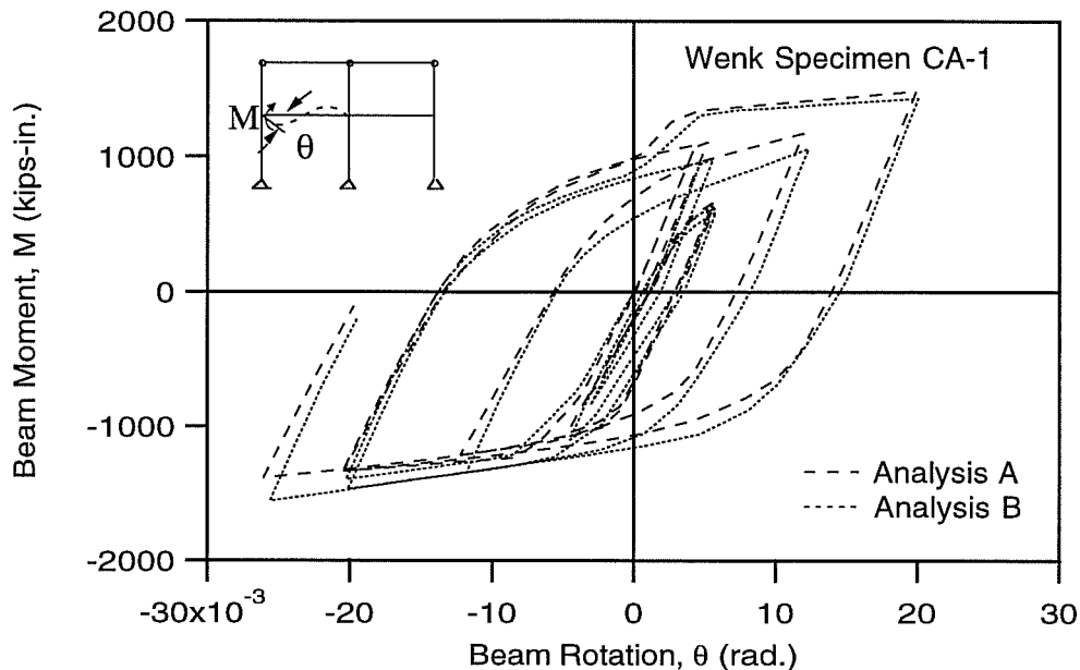
Fig. 7.24c: Comparison of Beam Moment-Rotation Relations of Left Composite Beam Obtained by the Analyses Using Different Methods to Consider Changing Inflection Point for Wenk Specimen CA-1 (Wenk 1977).
