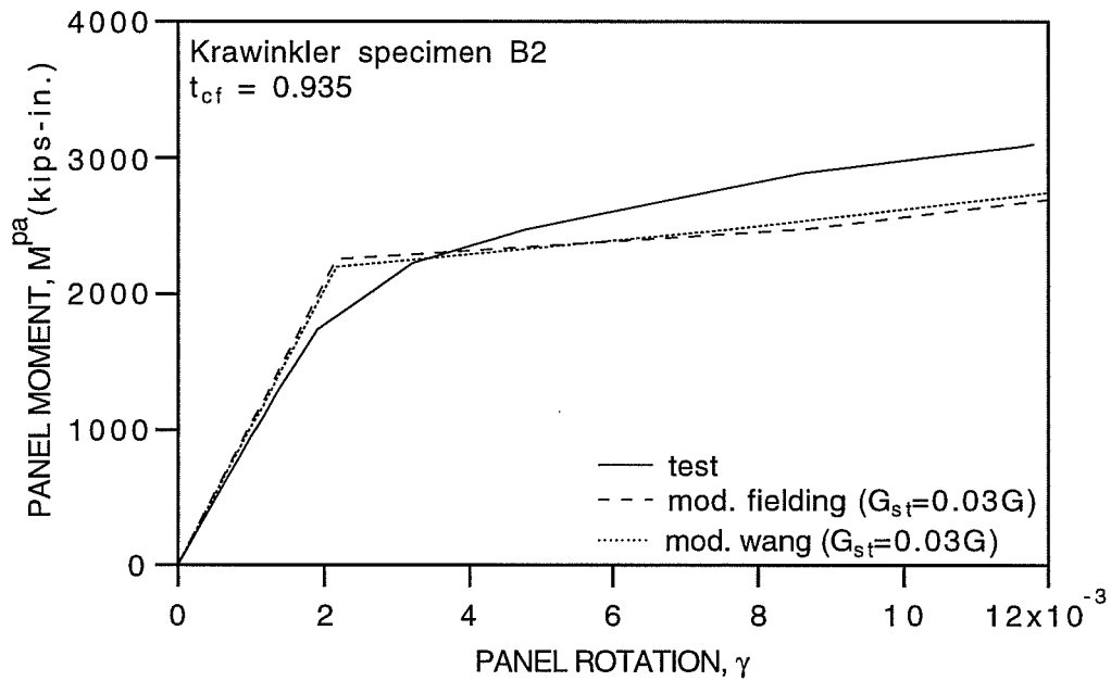
Fig. 5.18: Comparison of the Modified Models and Test Data for Krawinkler Specimen B2
