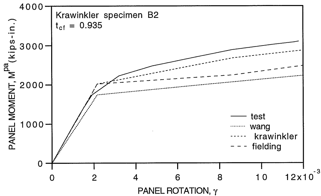
Fig. 5.8: Comparison of the Existing Models and Test Data for Krawinkler Specimen B2
