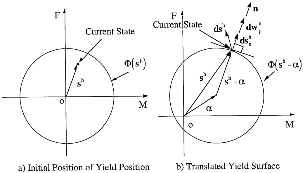
Fig. 2.6: Translation of Yield Surface and Normal Vector to Yield Surface
