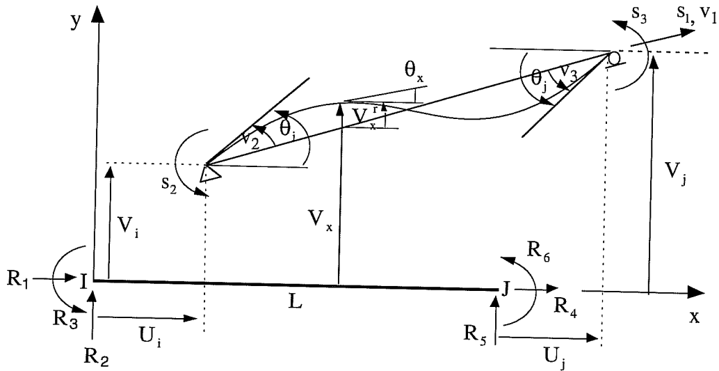
Fig. 3.2: Relative Displacements and Transverse Deflections
