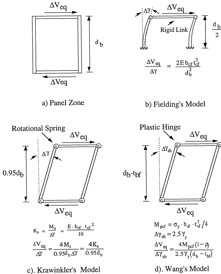
Fig. 5.5 Post Elastic Stiffness Models
