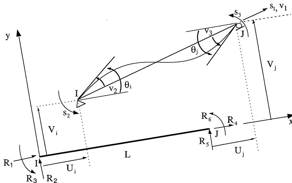
Fig. 2.5: Element Relative Forces and Deformations in Local Coordinate System
