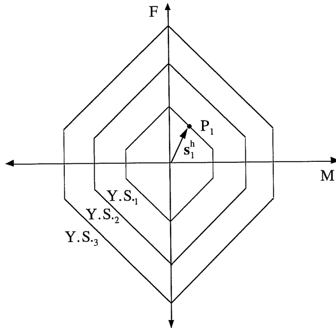
Fig. 2.9: Yield Surfaces Prior to Yielding
